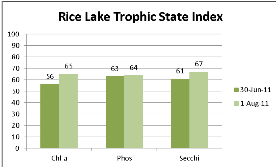
Figure 10: TSI
