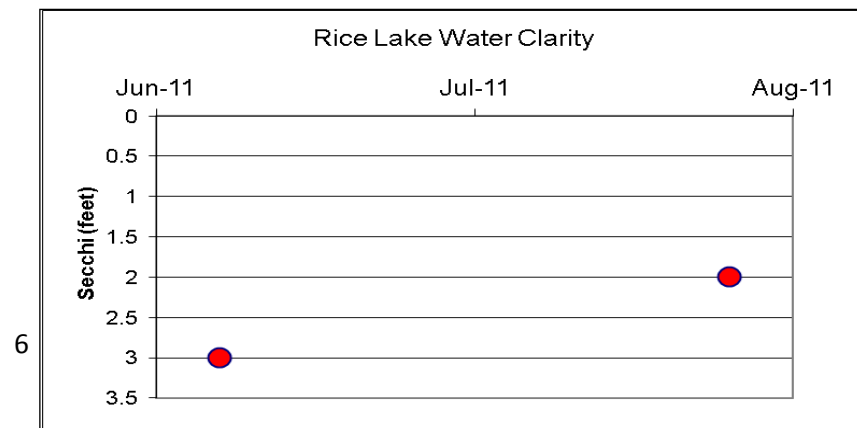
Figure 9: Secchi Measurements
