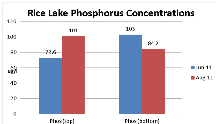
Figure 8: Total Phosphorus
