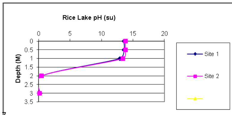
Figure 12: pH
