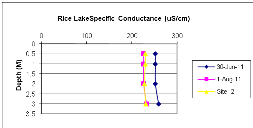
Figure 11: Specific Conductance
