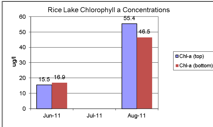
Figure 7: Chlorophyll a
