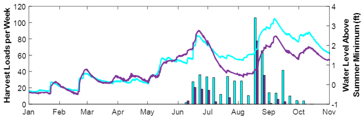
Figure 13: Aquatic plant harvesting loads removed in the Yahara River between Waubesa to Kegonsa (cyan bars) and Kegonsa to Stoughton (purple bars). Also, corresponding water levels above summer minimum are shown for Lake Waubesa (cyan) and Lake Kegonsa (purple).
